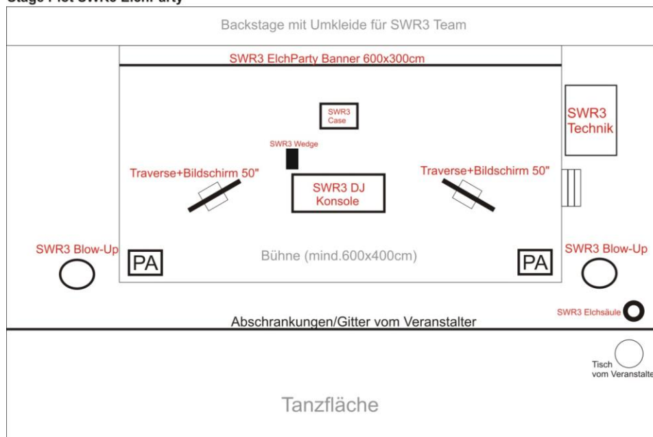
Stage Plot SWR3 ElchParty
